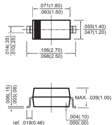
SOD-323
